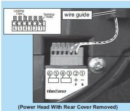
FIG 3-3 Insert wires.
