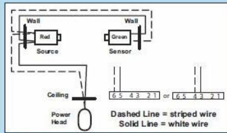
FIG. 4-5b Pre-Wired source and sensor wiring methods.
