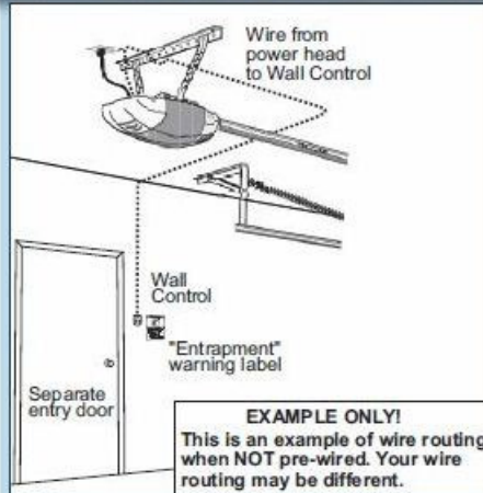
FIG. 3-1 Wall Control wire routing
