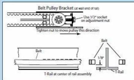
FIG. 1-7 Belt adjustment.
