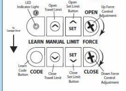
FIG. 6-1 Limit controls.
