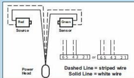
FIG 4-5a Source and sensor wiring methods.
