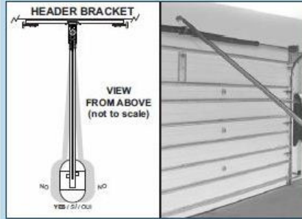
FIG. 2-4 Position assembly and align.
